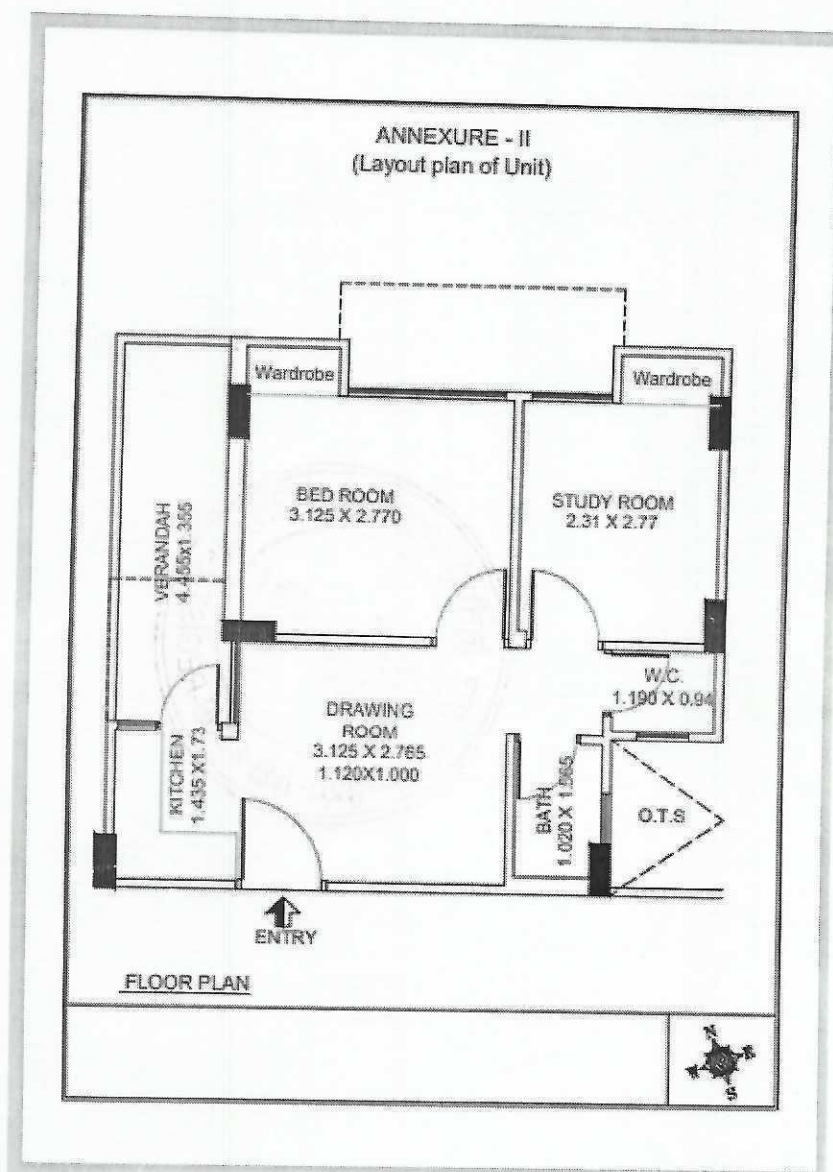
LAYOUT PLAN OF THE UNIT NO 12 AND THE COMPLEX
