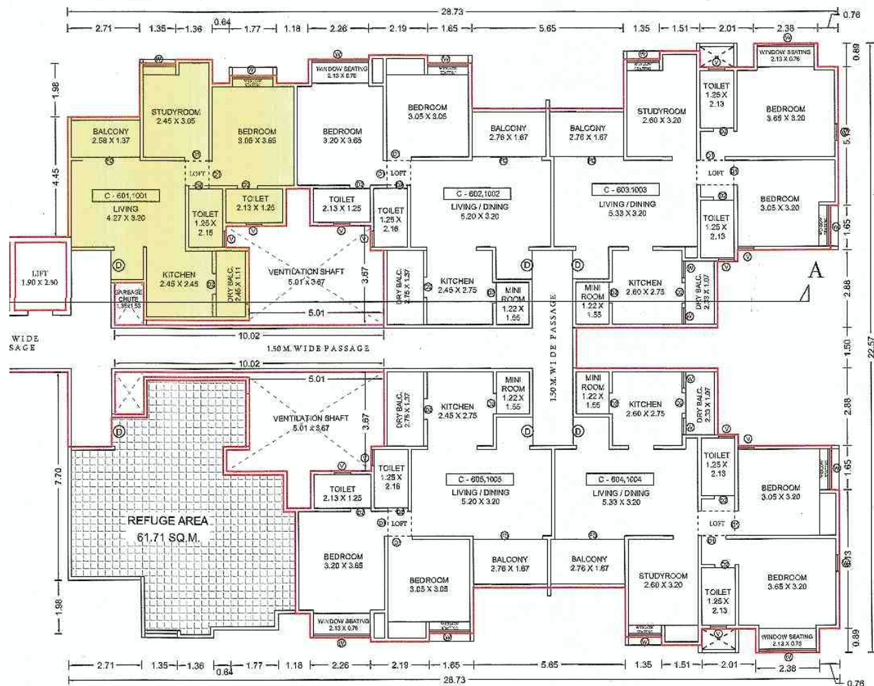
TYPICAL - 6 & 10 FLOOR PLAN
