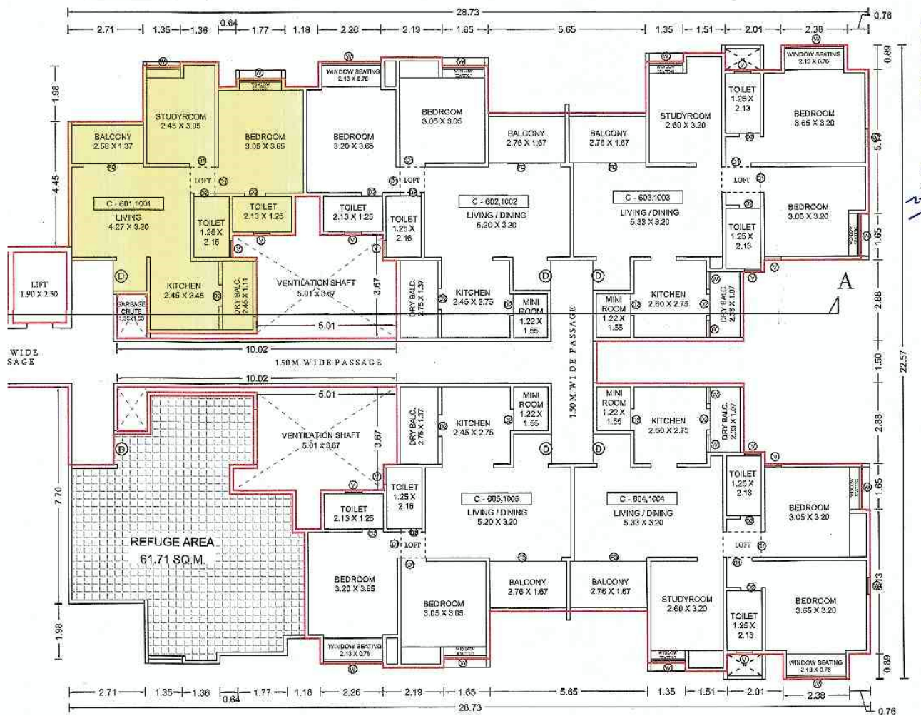
TYPICAL - 6 & 10 FLOOR PLAN
