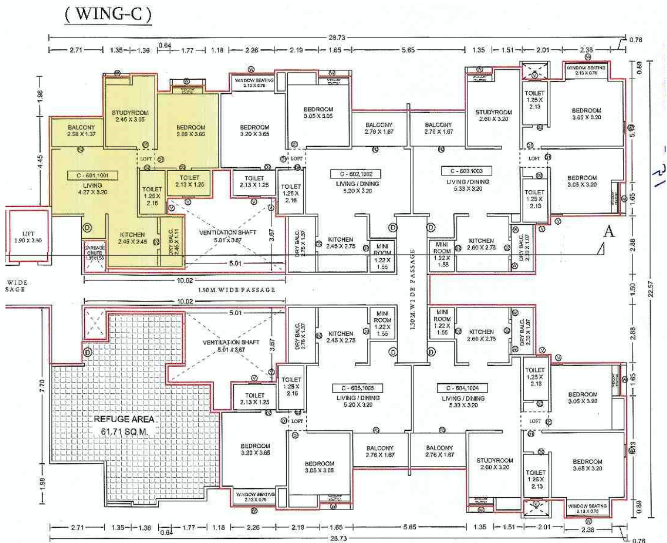
TYPICAL - 6 & 10 FLOOR PLAN WING - C FLAT NO.
