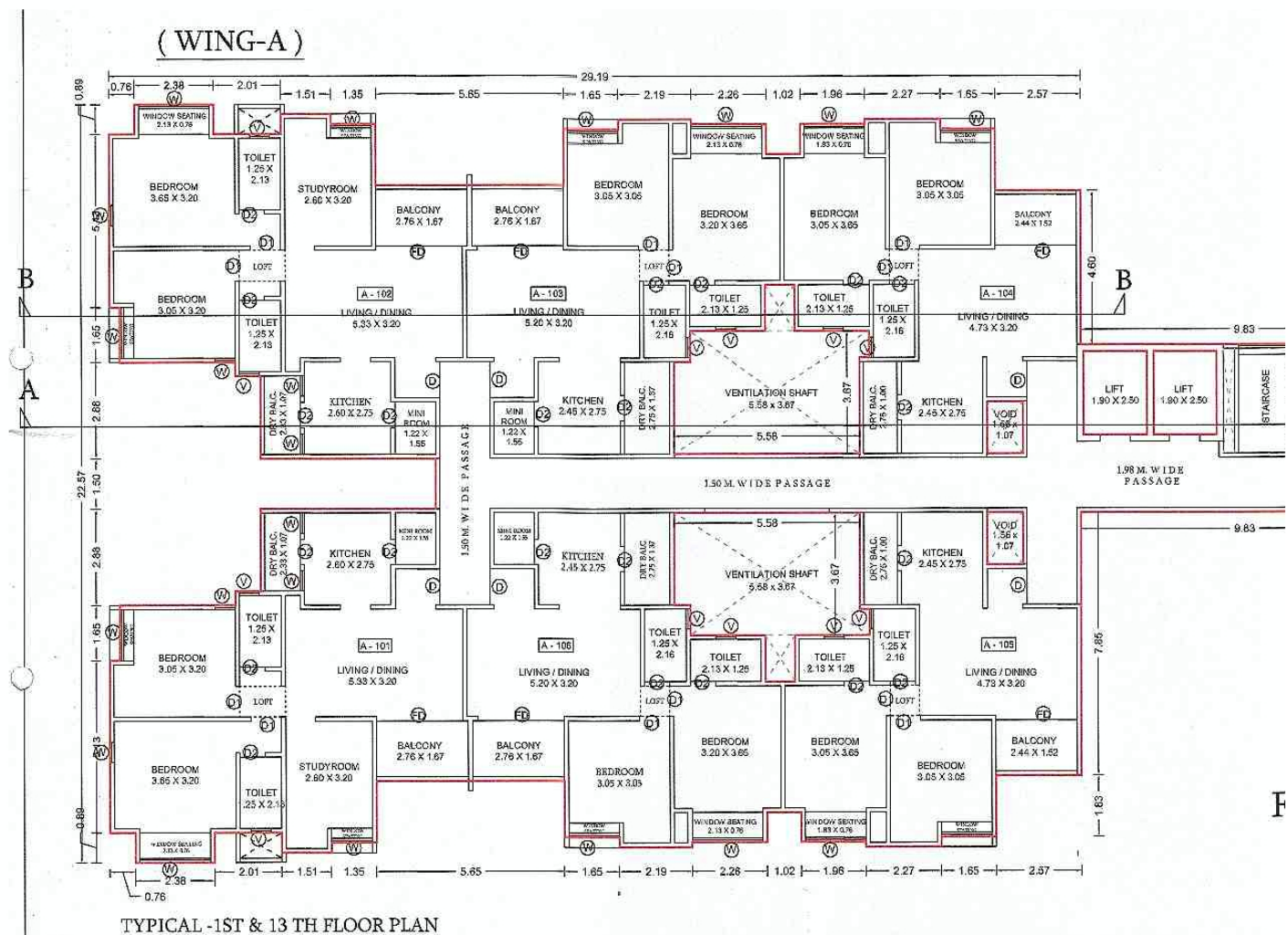
TYPICAL -1ST & 13 TH FLOOR PLAN
